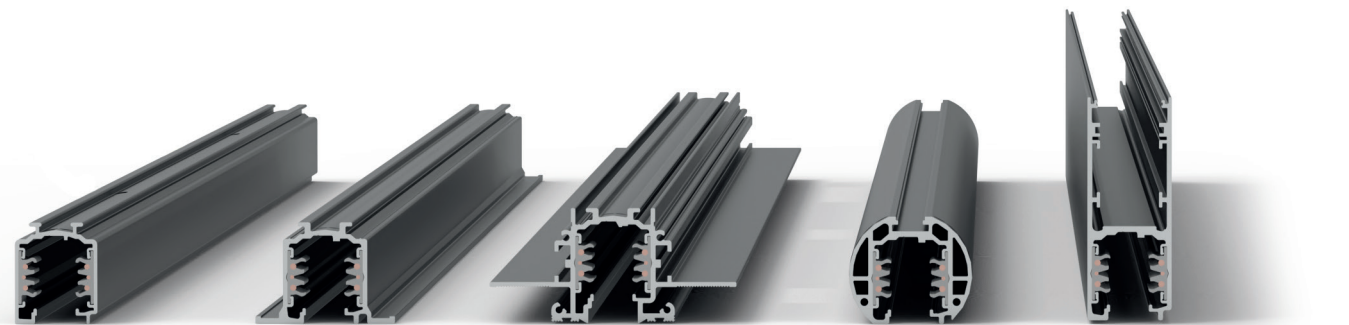
OneTrack OneTrack Recessed Lytespan Trimless Recessed* Lytespan Round Track* Lytespan H-Track*
